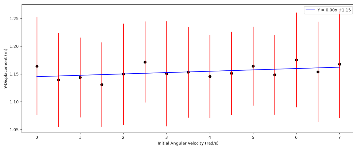
Figure 9: A graph of final y displacement of the curling stone against initial angular velocity. Each point is the average of 50 results with the standard deviation plotted as error bars, and a weighted line of best fit.
