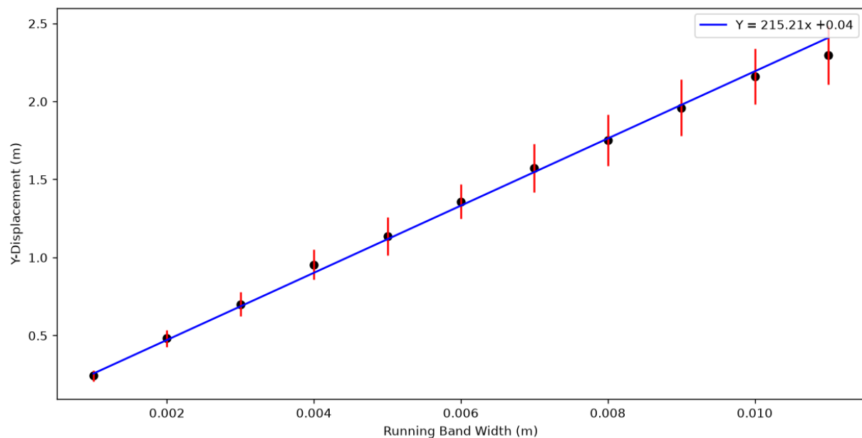
Figure 4: A graph of final y displacement of the curling stone against running band width, where each point is averaged from 50 results with the standard deviation plotted as error bars. A weighted line of best fit is plotted in blue.
