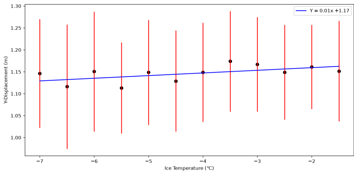
Figure 8: A graph of the final y displacement of the curling stone against the temperature of the ice, each point is the average of 50 results with the standard deviation plotted as the error bars and a weighted line of best fit.
