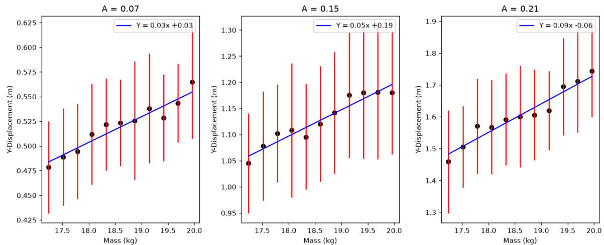
Figure 2: Graphs showing final y displacement of the curling stone against mass, for 3 different values of A. Each point is the average of 50 values, with a standard deviation and weighted lines of best fit.
